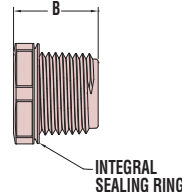
Threaded Vent Plug
